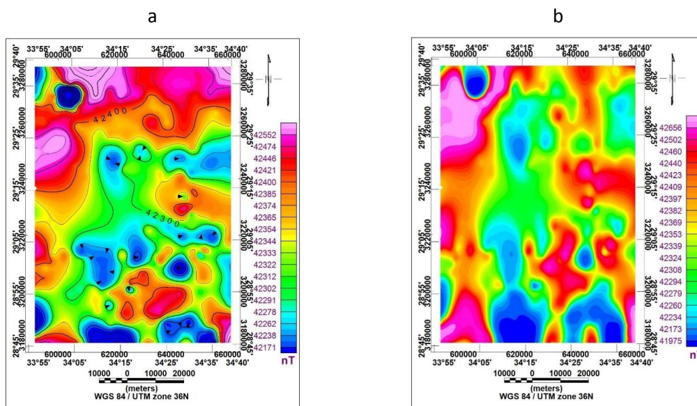
Fig.5, a: Total intensity magnetic map, b: Total intensity magnetic map reduced to the Pole (RTP map).
