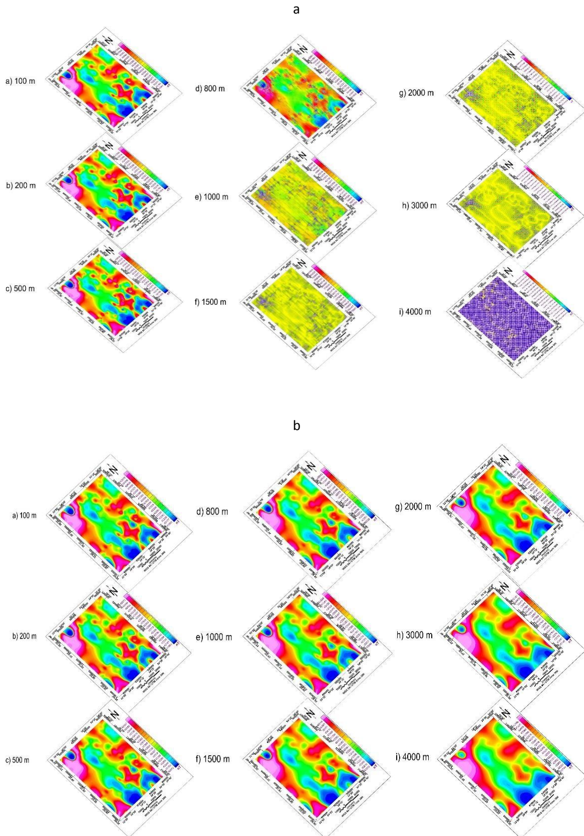
Fig.6, part1: represents the downward continuation at distances 100, 200, 500, 800, 1000, 1500, 2000, 3000 and 4000 m, Part2: represents the upward continuation at distances 100, 200, 500, 800, 1000, 1500, 2000, 3000 and 4000 m.
