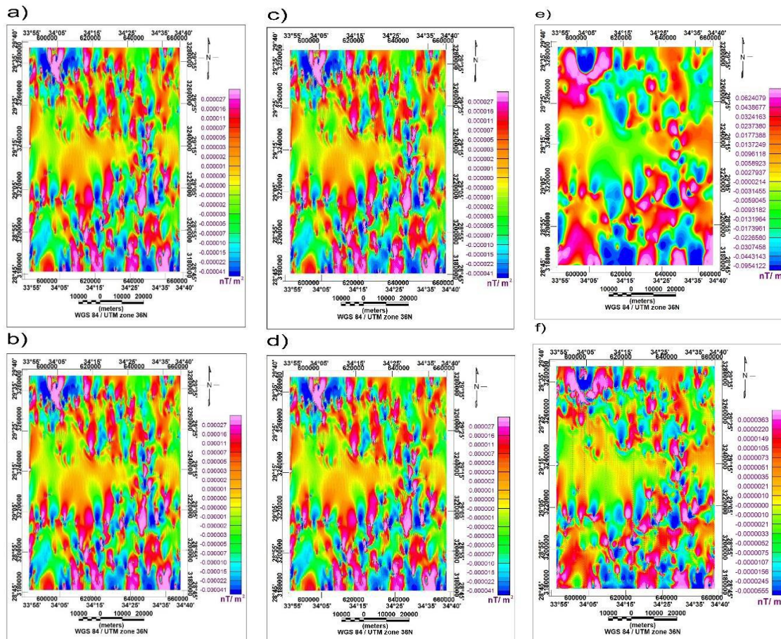
Fig.7: a) first horizontal derivative of RTP map in X-direction b) first horizontal derivative of RTP map in Y-direction c) second horizontal derivative of RTP map in X-direction d) second horizontal derivative of RTP map in Y-direction e) first vertical derivative of RTP map in Z-direction f) second vertical derivative of RTP map in Z-direction
