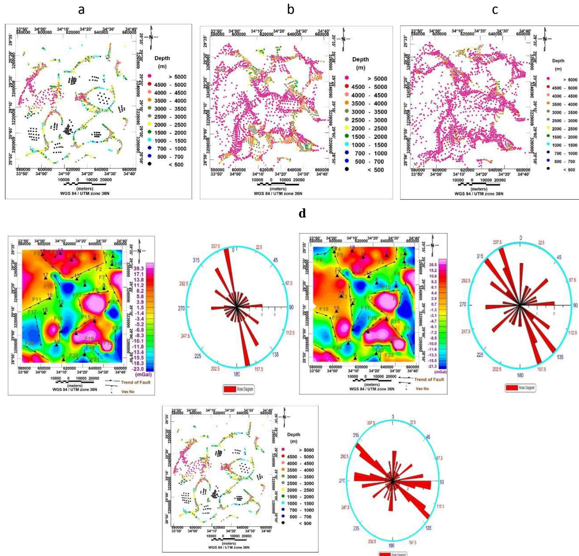
Fig.4, a: Euler solutions of structural index = 0, b: Euler solutions of structural index = 1, c: Euler solutions of structural index = 2, d: Fault elements dissecting the studied area from gravity interpretation, h pass and Euler solutions with structural index zero and Major trend faults dissecting the studied area.
