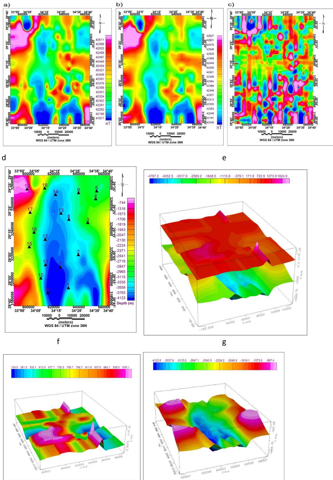
Fig.8, a: Observed magnetic anomaly, b: calculated magnetic and c: error percentage, d: basement relief map,e: 3-D view map, f: Topographic – depth map and g: Basement – depth map.
