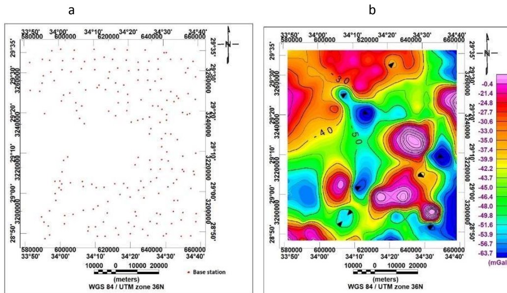
Fig.2, a: Gravity stations in the studied area, b: Bouguer anomaly map of the studied area.
