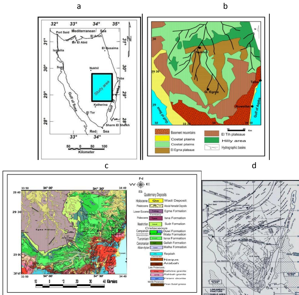
Fig.1, a : Location map of the studied area, b: Geomorphc Map of Sinai (after Abd Allah and Abu Khadrah, 1977), c: Geologic map of the studied area (modified after UNSECO Cairo Office 2005), d: Tectonic Map of Sinai Peninsula (after Neev, 1975 and Agah, 1981)..
