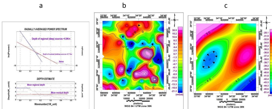
Fig.3, a: Power spectrum of gravity data showing the corresponding averaging regional and the residual, b: Regional Bouguer anomaly map and b: residual Bouguer anomaly map using a low- and high-pass filter with a cut wave number of 0.018 km -1 .
