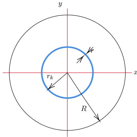
Fig. 3. Moment of inertia of a circular disc
