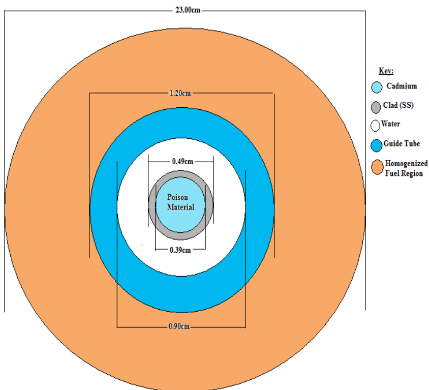
Fig. 2. Description of the control model for NIRR-1 core
