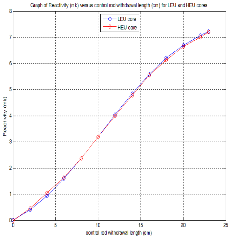
Fig. 6. Reactivity (mk) versus control rod withdrawal length (cm) of the active fuel region
