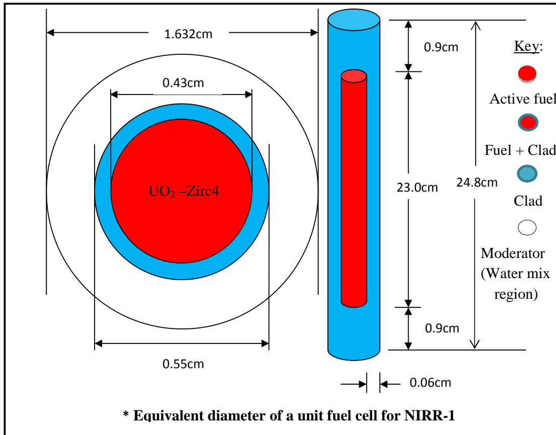
Fig. 1. The height and diameter of the active fuel cell and fuel rod models for the potential LEU core for NIRR-1
