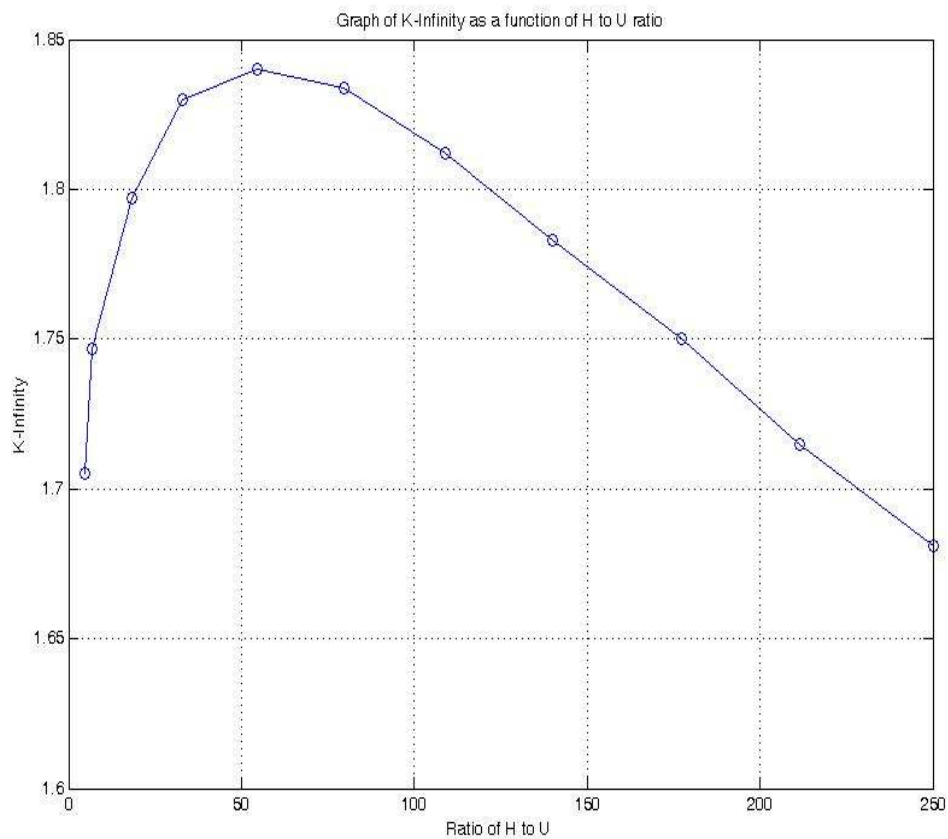
Fig. 5. Plot of k-infinity as a function of H to U ratio for the HEU (90.2% UAl 4 ) core
