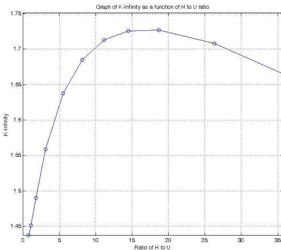
Fig. 4. Plot of k-infinity as a function of H to U ratio for the LEU (19.75% UO 2 ) core
