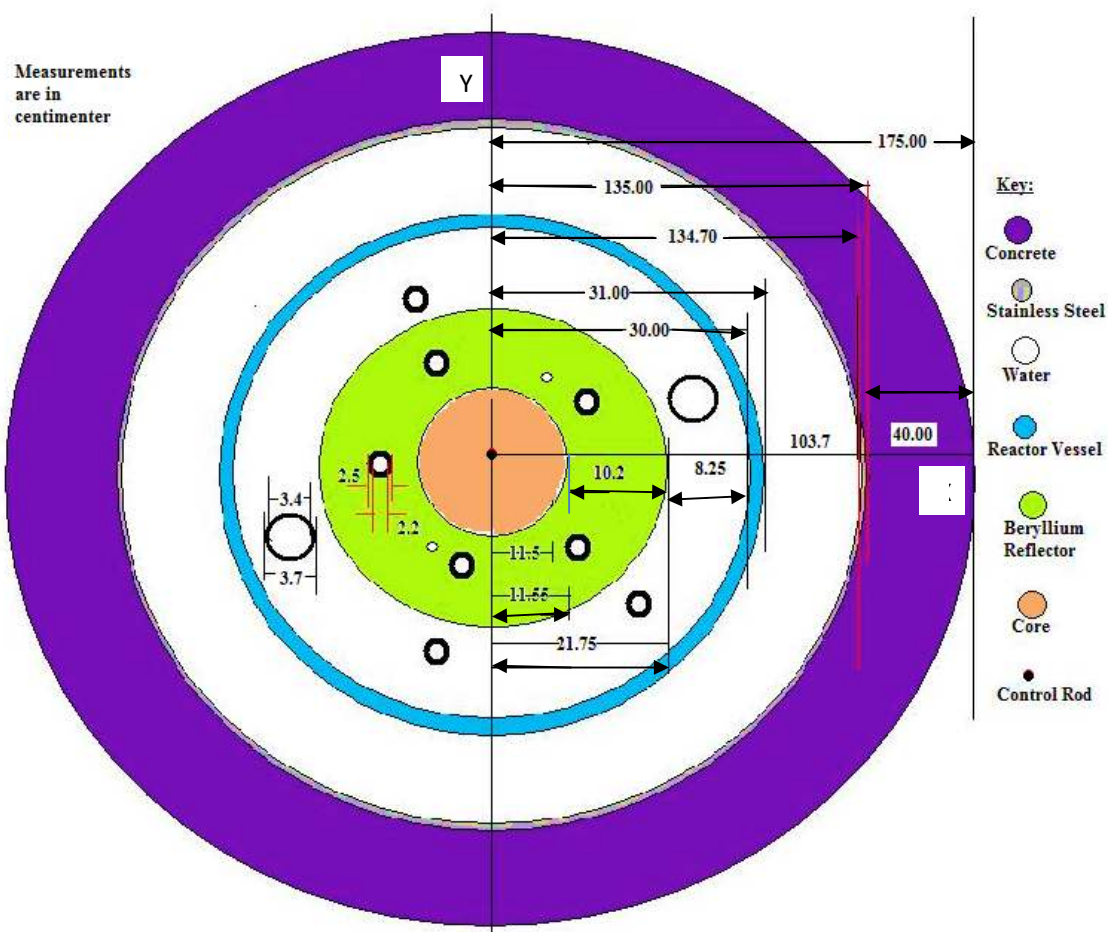
Fig. 3. The geometry and dimensions of various components of NIRR-1 core
