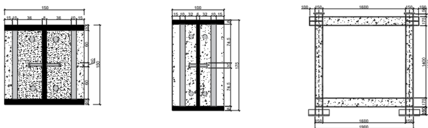
Fig. 2. Flanges of the PEC components
