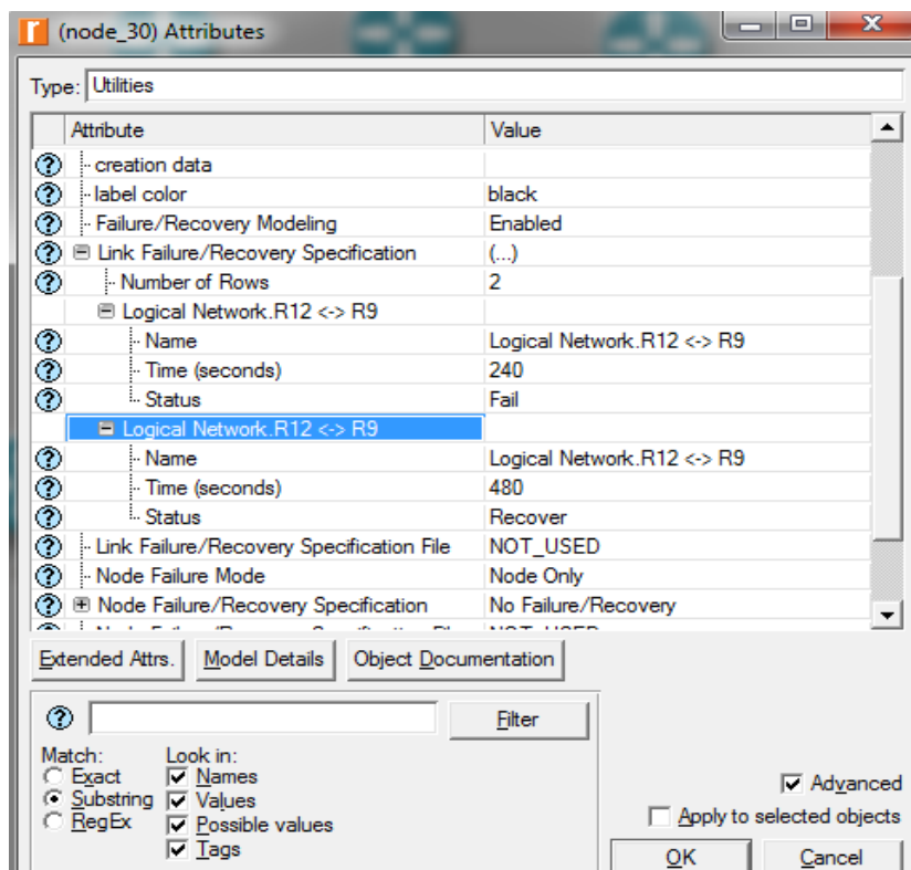
Fig. 4. Configuration for failure recovery
